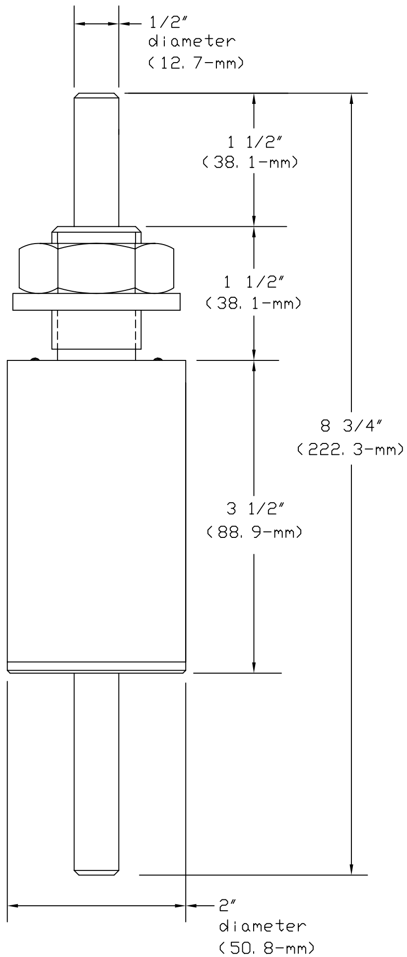
1/2" Diameter Ball Bearing Rotary Feedthrough Part No. 8610 1050 0000
