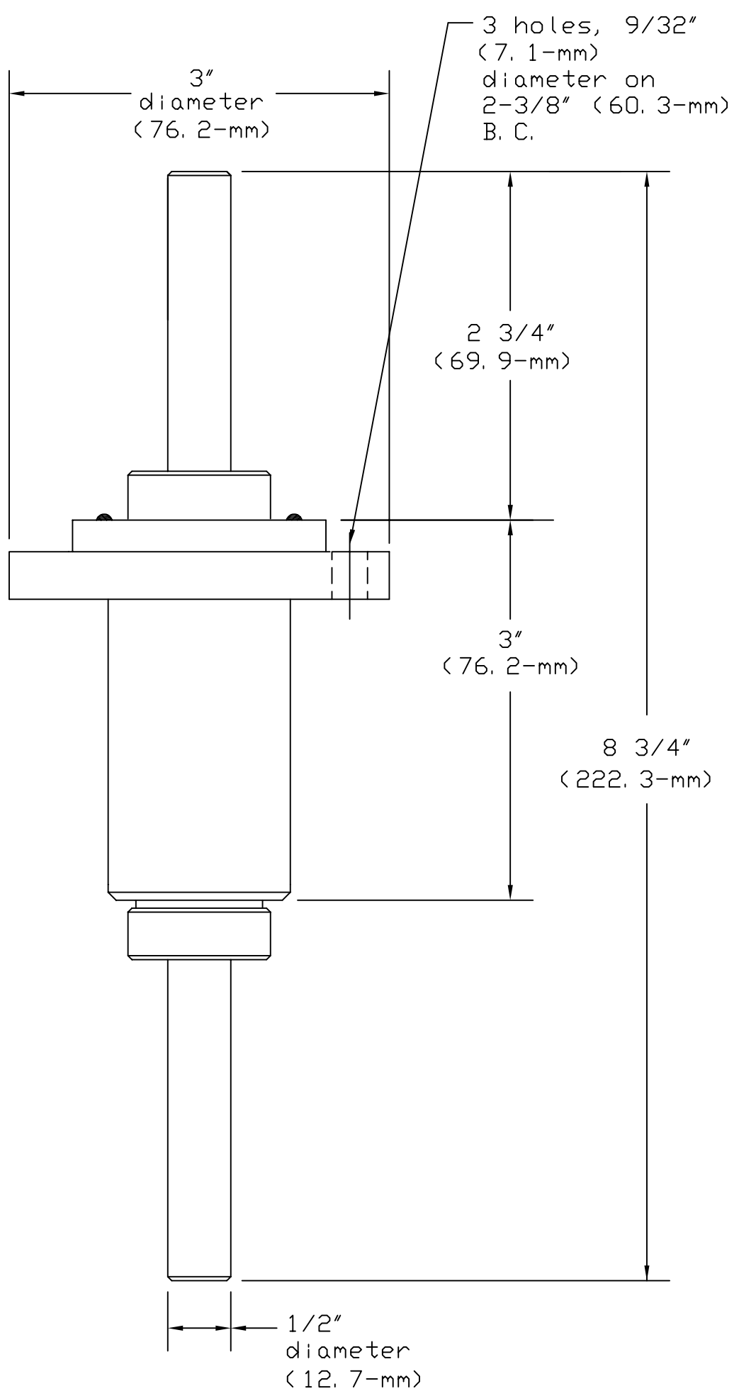
1/2" Diameter Ball Bearing Rotary Feedthrough (flanged) Part No. 8610 1150 0000
