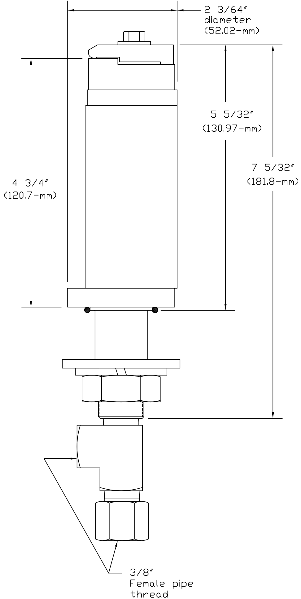
3000 Ampere High Current Evaporation Boat/Filament Feedthrough Part No. 8620 1011 0000
